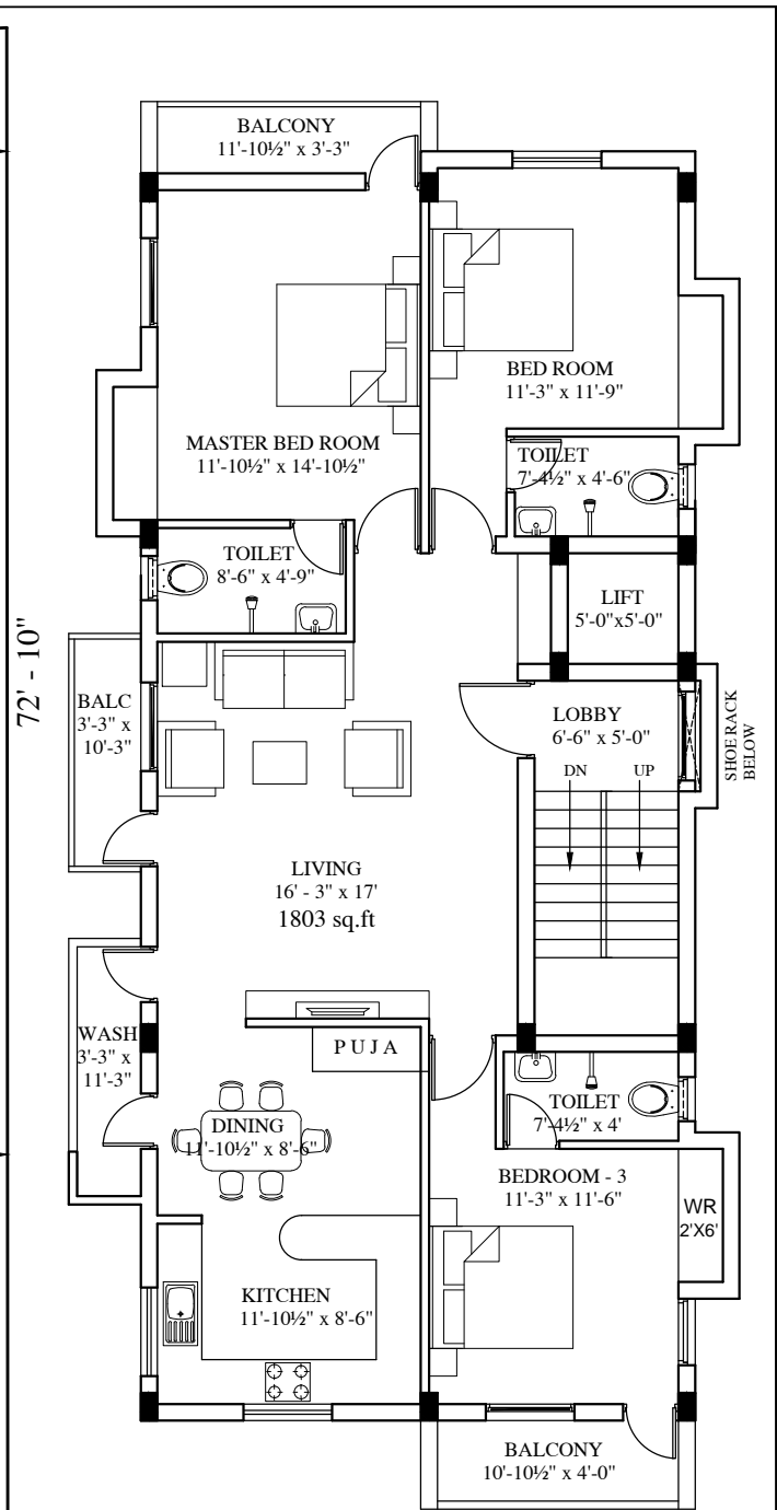
TYPICAL FLOOR PLAN [I,II & III]
